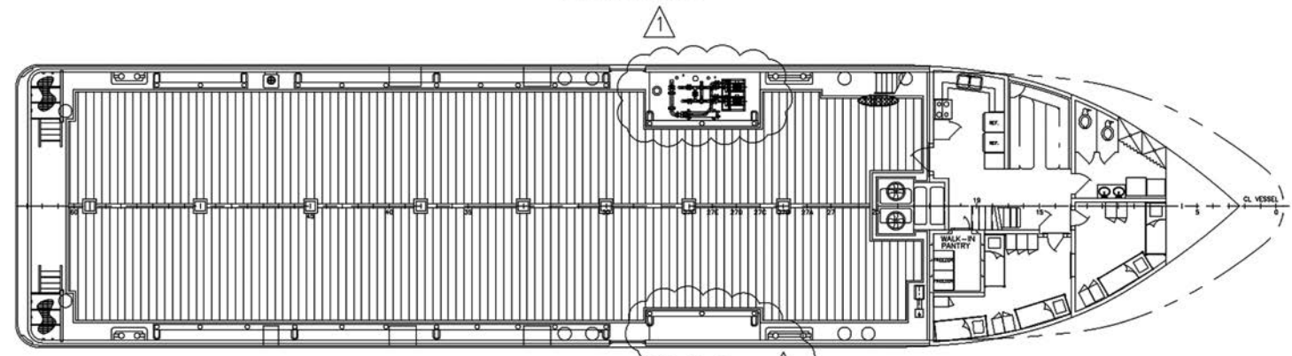
MAIN DECK ARRANGEMENT
