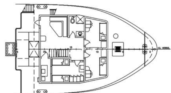
FOCSLE DECK ARRANGEMENT
