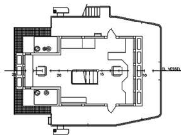
PILOTHOUSE ARRANGEMENT
