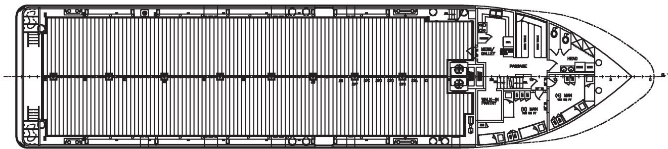
MAIN DECK ARRANGEMENT
