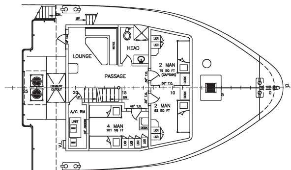
FOC SLE DECK ARRANGEMENT
