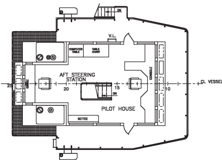
PILOTHOUSE ARRANGEMENT
