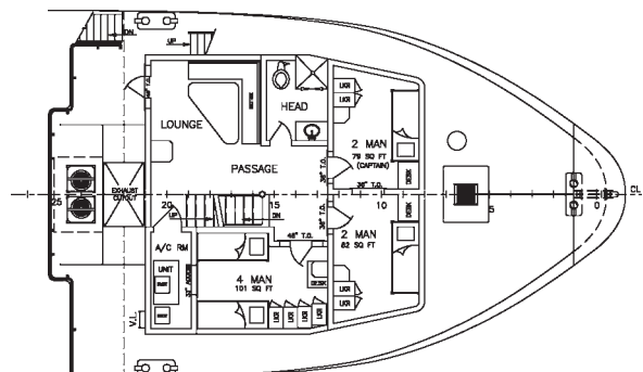
FOCSLE DECK ARRANGEMENT
