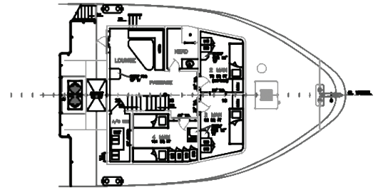
FOCSLE DECK ARRANGEMENT
